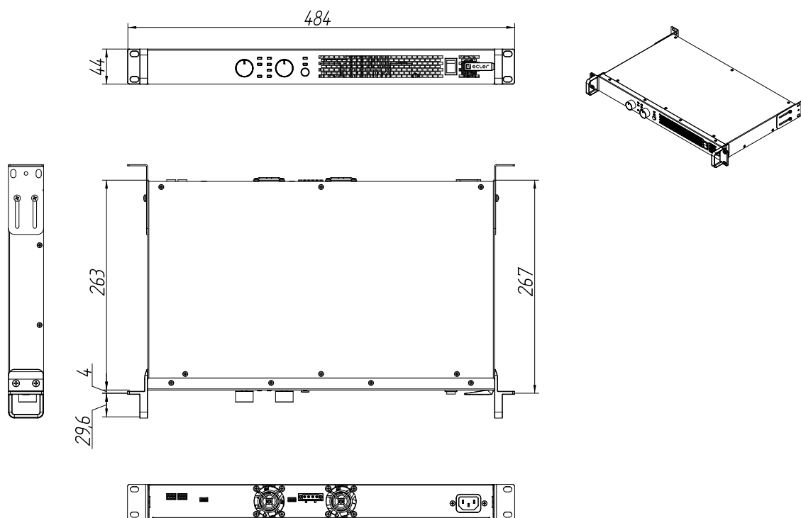
Ecler AURA-2BI50 Mechanical Diagram
