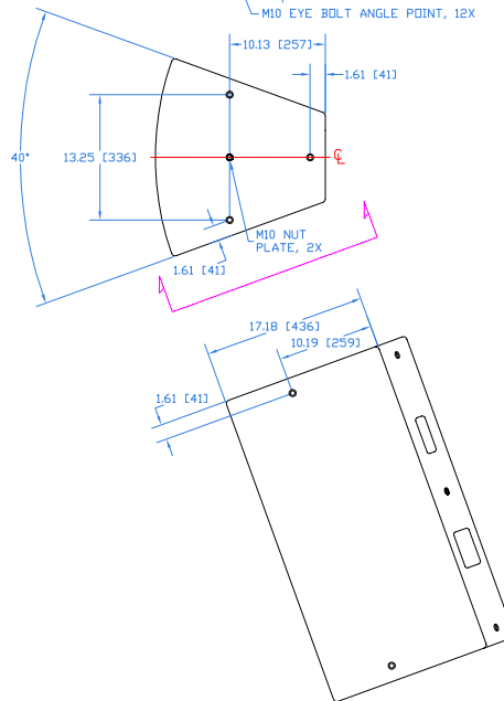
GRILLE PARTIALLY SHOWN
