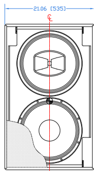
GRILLE PARTIALLY SHOWN
